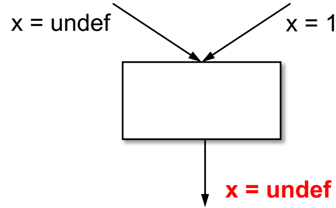
Uninitialized Variables
