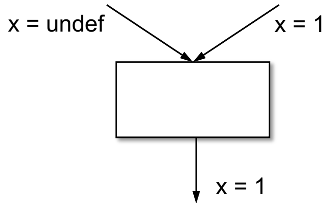
Constant Propagation
